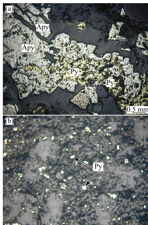
Fig. 3 Microstructure feature of pyrite in Dachang tin-polymetallic ore-field, Guangxi, China: (a) Replacement of pyrite by arsenopyrite; (b) Disseminated texture of pyrite
