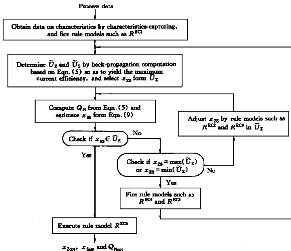
Fig.2 Flow chart of reasoning using combination of backpropagation networks and rule models
