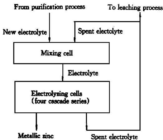
Fig.1 Electrolytic process
